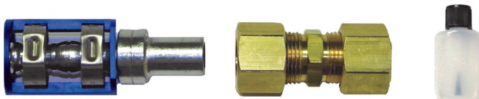
Kits include compression union (1), rubber hose adapter (1), clamp holder (1), clamps (2), and sealant (1)
