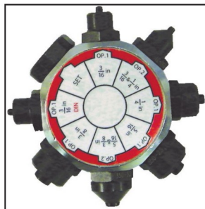
"Dial-A-Size" turret
